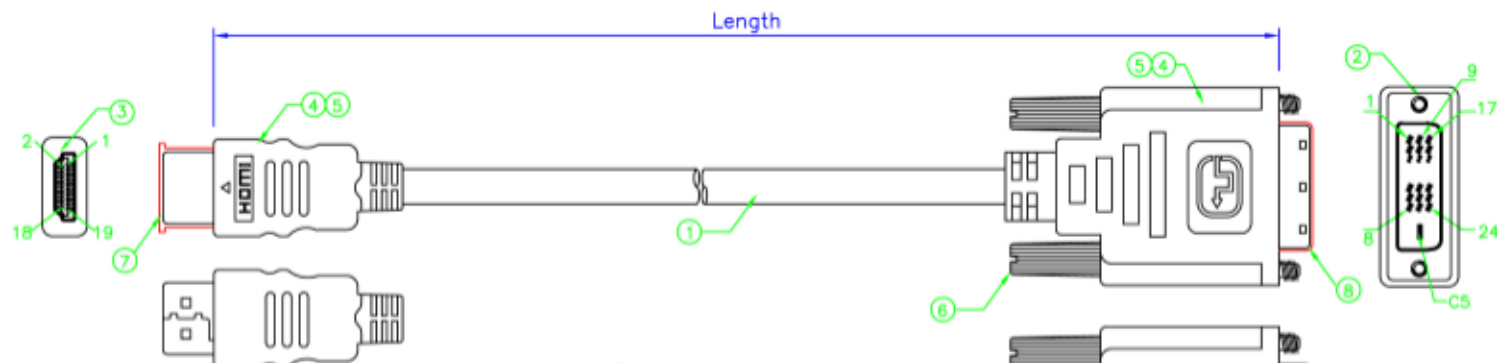
Pin Assignment
