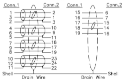
Pin Assignment
